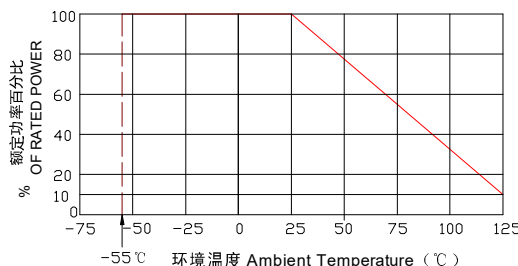
Derating curve of coaxial attenuator
